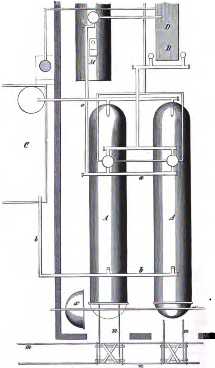
Fig. 309.—Creosoting cylinders.
